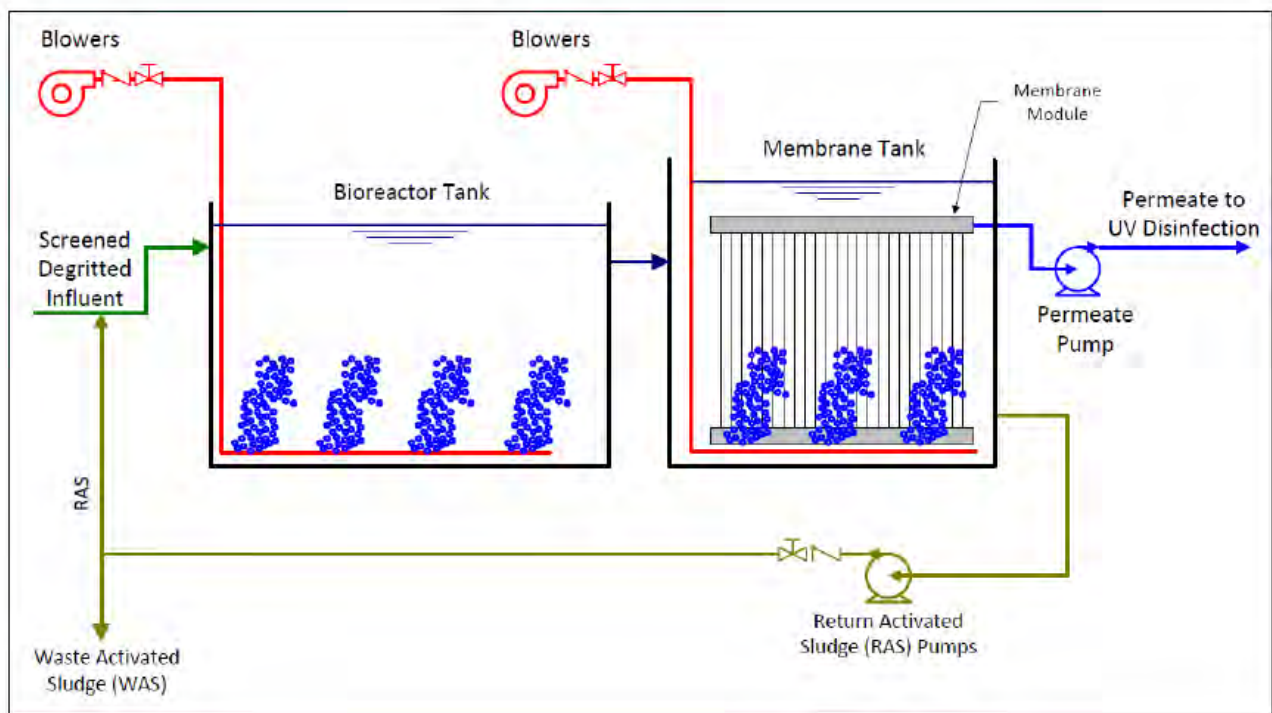
Figure 9: Typical MBR Operation
