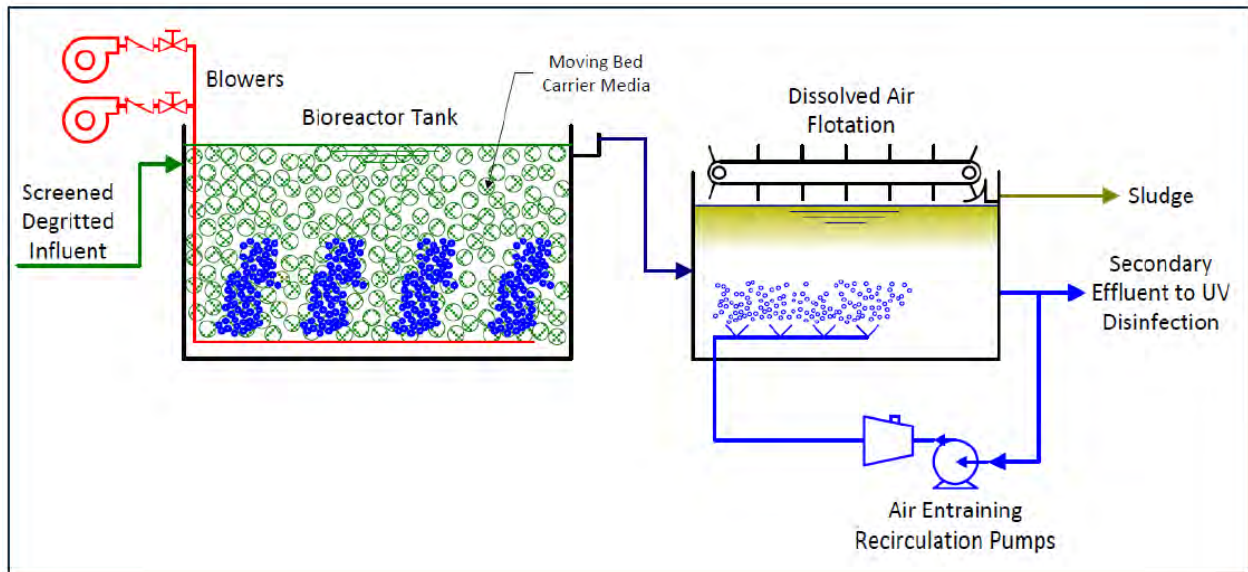
Figure 3: Typical MBBR and DAF Schematic
